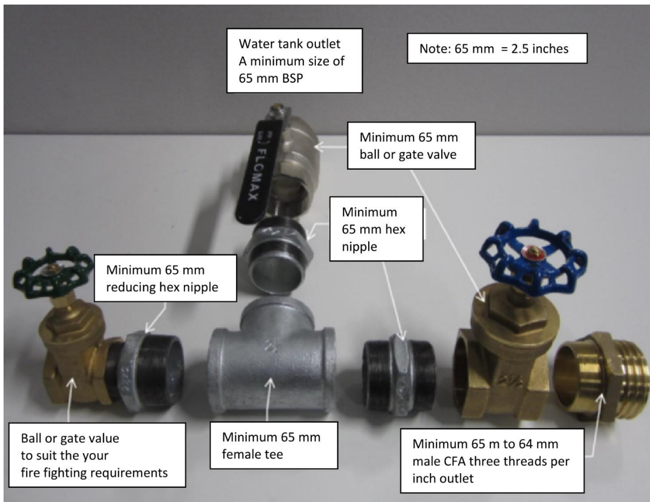
Figure 1: Common tank fittings
