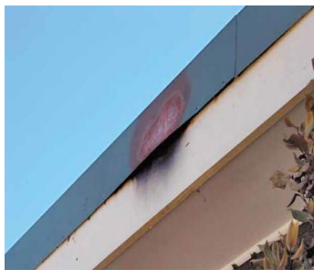
Eaves, Gutters & Downpipes – Up to and including BAL 29 Protect eaves penetrations as per roof penetrations.
