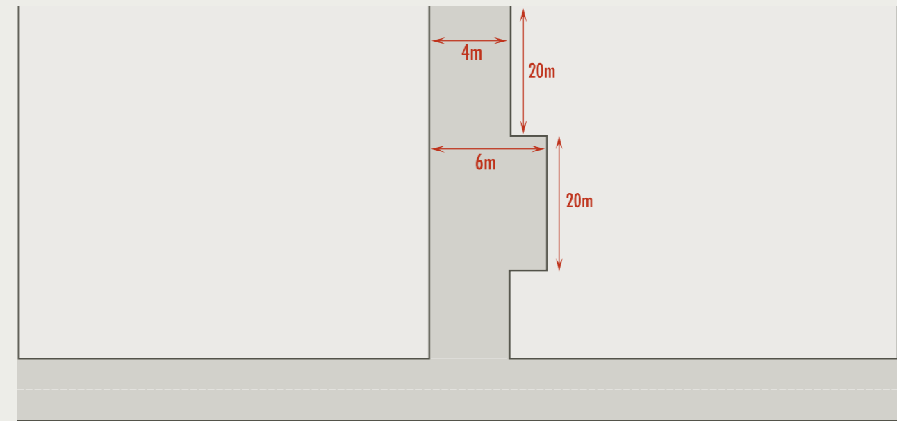
Figure 18 – Access road length/passing bays
