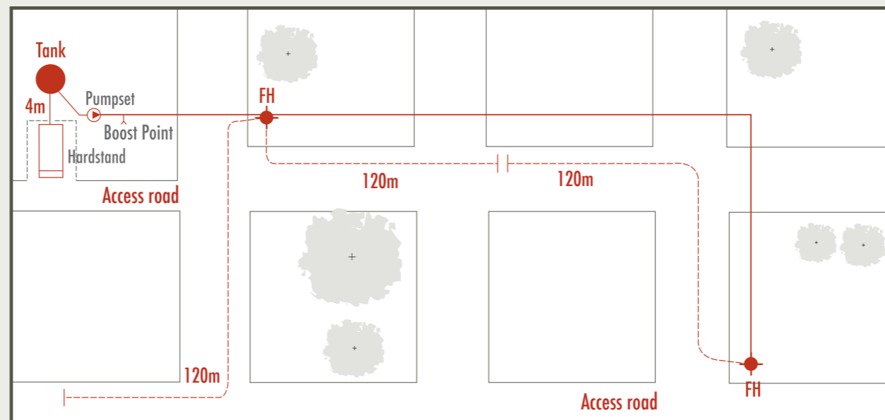
Figure 23 – Static water storage coverage, with reticulation
