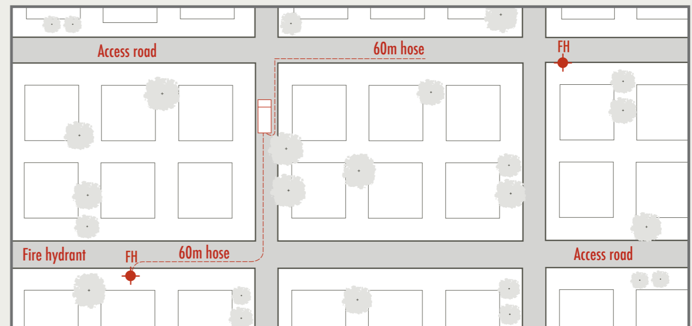
Figure 20 – Reticulated fire hydrant coverage
