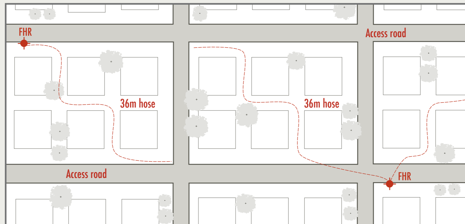
Figure 19 – Fire hose reel (FHR) coverage
