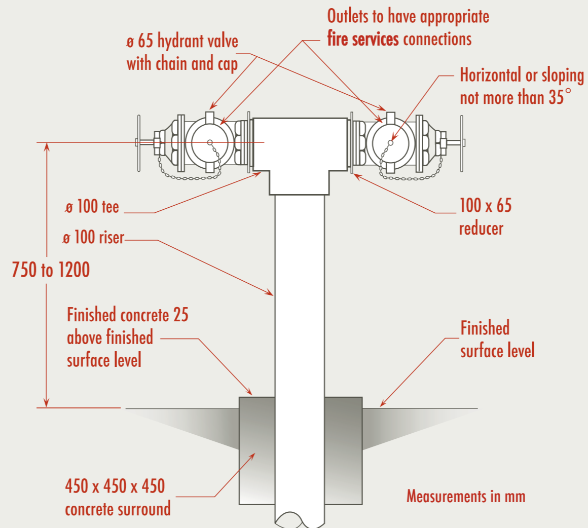
Figure 21 – External fire hydrant pursuant to AS 2419.1
