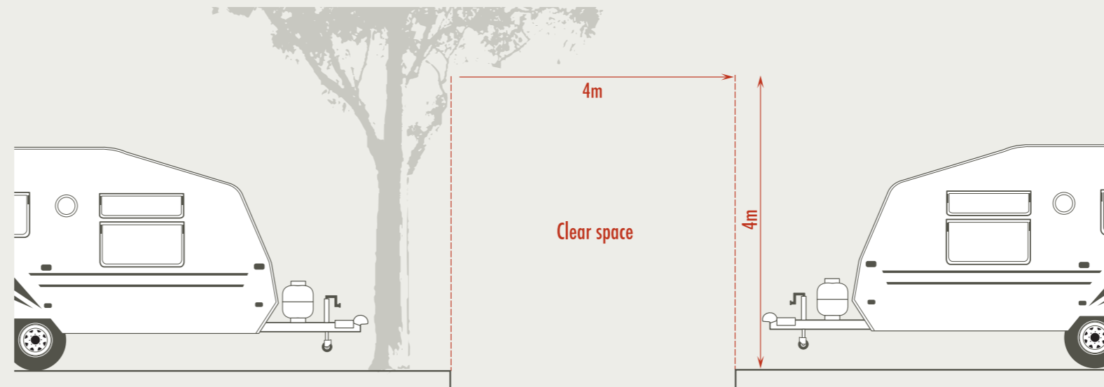
Figure 16 – Trafficable width and height
